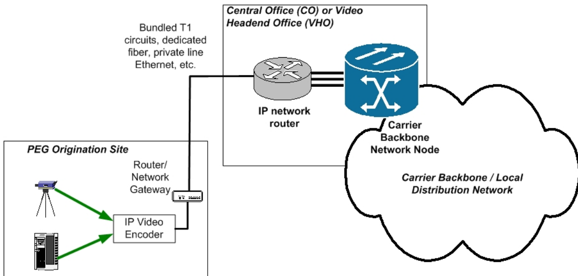
Figure 1: PEG Origination Uplink
