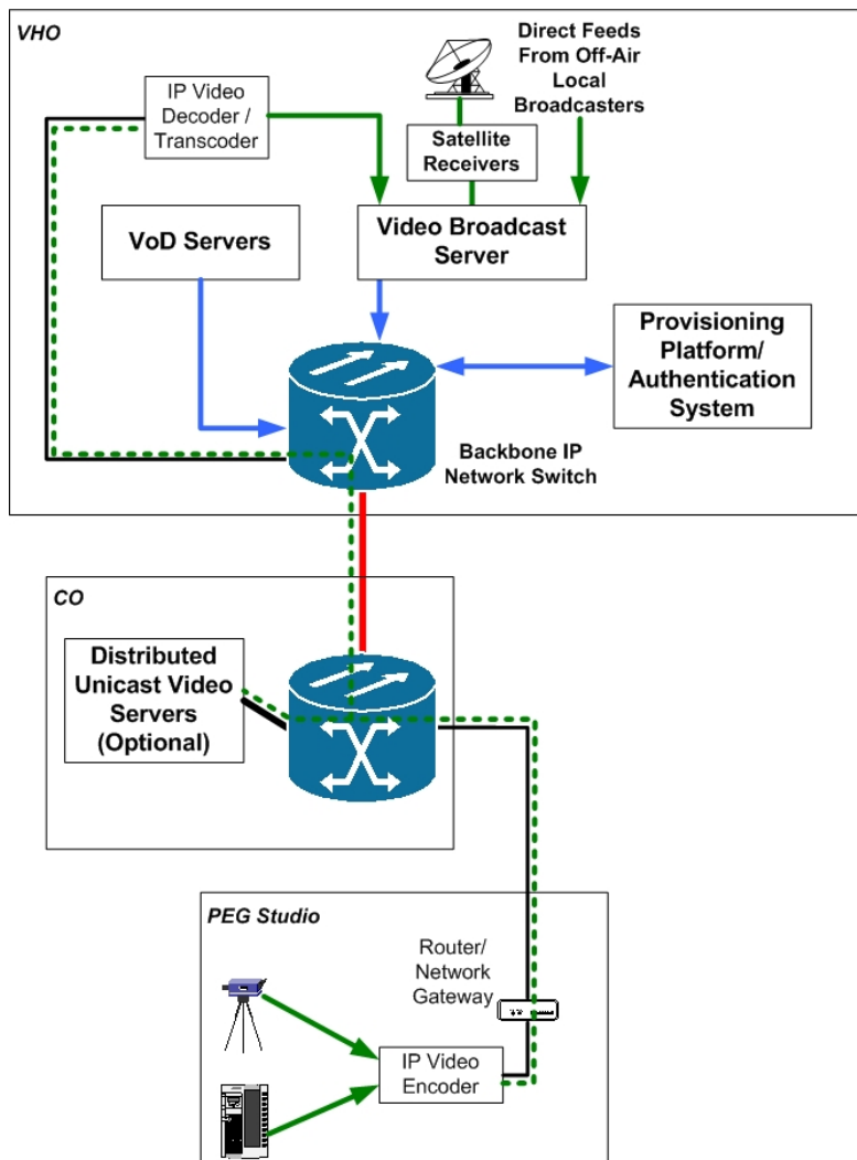
Figure 2: PEG Channel “Insertion”
